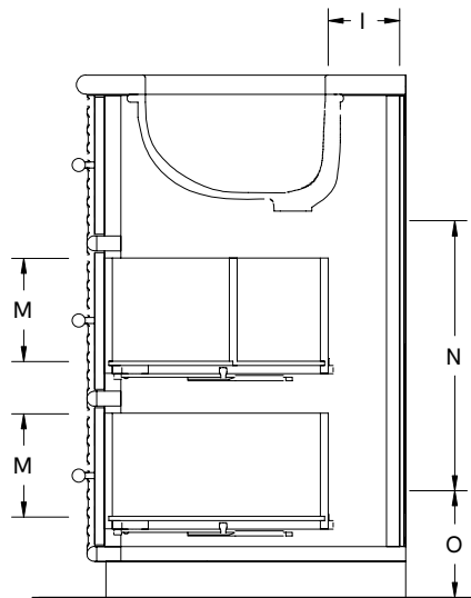
Section
